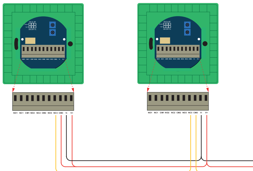
Maasland handmelder 330PGL
